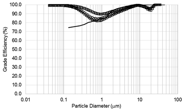
Fig. 9. Theoretical and experimental grade efficiencies. Series with “ \Delta ” for C_{in} = 121 \text{ mg/m}^3 , series with “ * ” for C_{in} = 363 \text{ mg/m}^3 , series with “ \square ” for C_{in} = 1231 \text{ mg/m}^3 and series with solid line plots the PACyc results for C_{in} = 572 \text{ mg/m}^3 .
