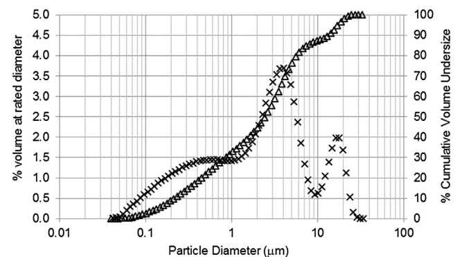
Fig. 4. Particle size distribution in feed. The series with the “x” plots the % volume at rated diameter and the series with the “Δ” plots the cumulative volume undersize.
