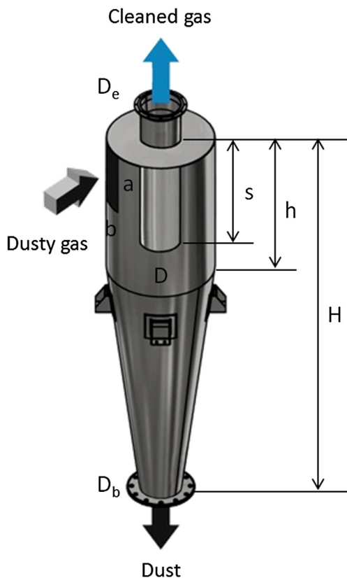
Fig. 1. Typical reverse-flow cyclone.
