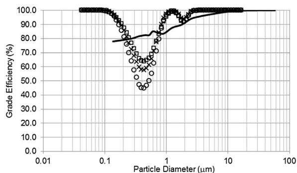
Fig. 5. Theoretical and experimental grade efficiencies. Series with "x" plots the grade efficiencies for C_{in} = 84 \text{ mg/m}^3 , series with "o" for C_{in} = 450 \text{ mg/m}^3 , series with the "□" for C_{in} = 584 \text{ mg/m}^3 . The series with solid line plots the PACyc results for C_{in} = 429 \text{ mg/m}^3 .
