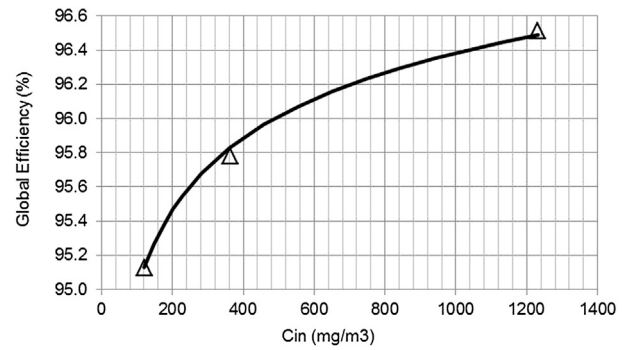
Fig. 11. Series with “ \Delta ” plots the experimental global efficiencies in function of the inlet concentration and the series with solid line plots the global efficiencies obtained through the Smolik model with k = 0.141 .
