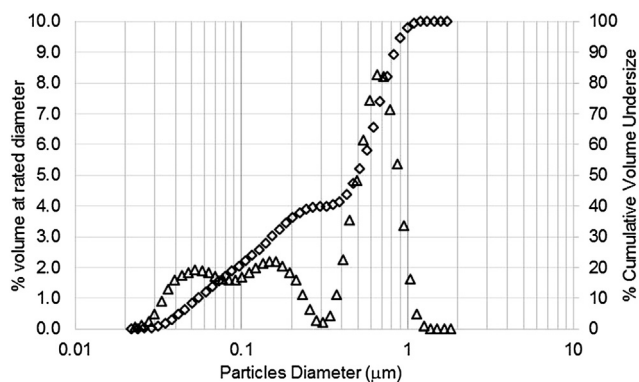
Fig. 14. Particle size distribution at the outlet of the pilot rig. Series with the “Δ” plots the outlet distribution for C_{in} = 362 \text{ mg/m}^3 . Series with the “◇” plots the cumulative volume undersize for C_{in} = 362 \text{ mg/m}^3 .
