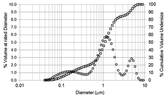
Fig. 12. Particle size distribution in feed. Series with “ * ” plots the % volume at rated diameter and the series with the “ \square ” plots the cumulative volume undersize.
