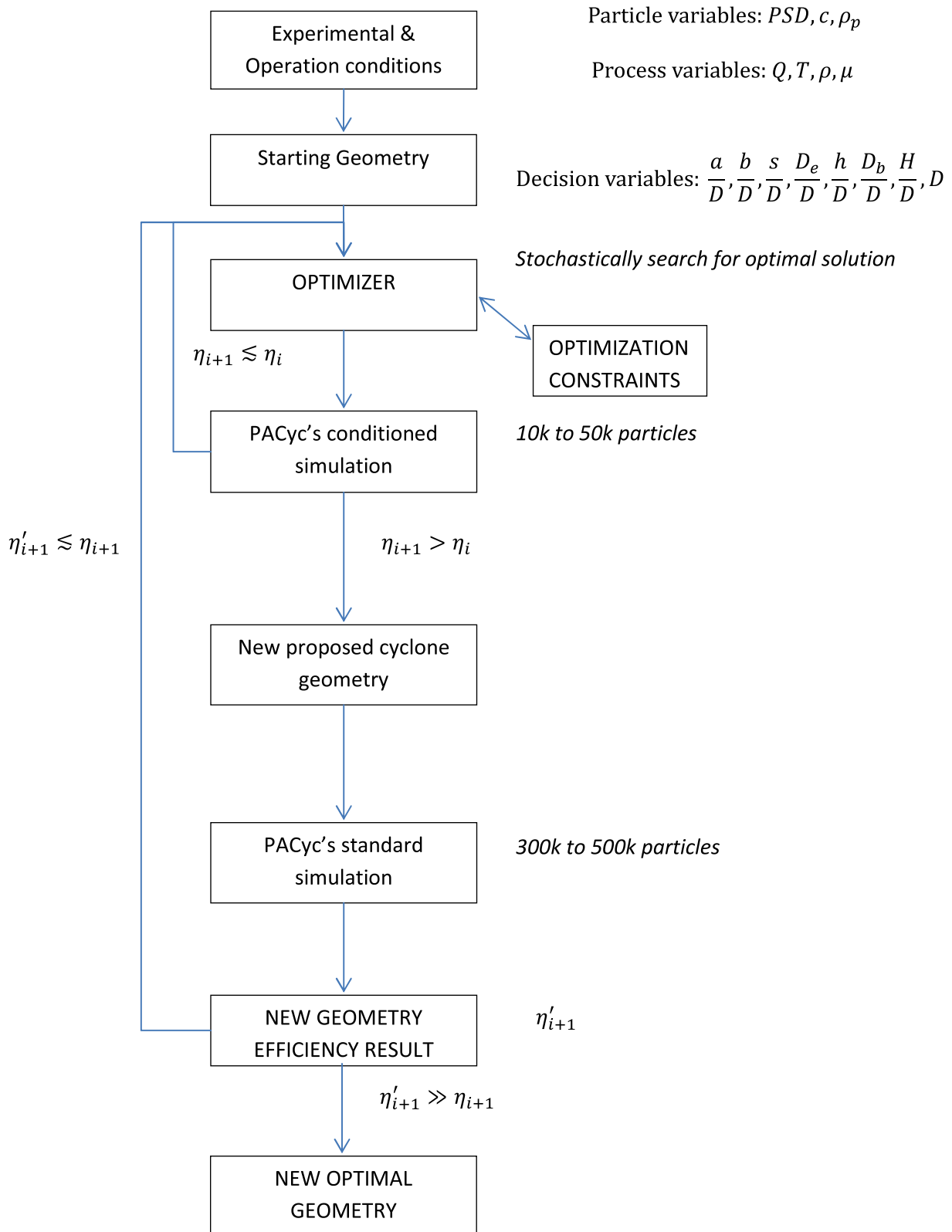
Fig. 2. Optimization flow sheet.
