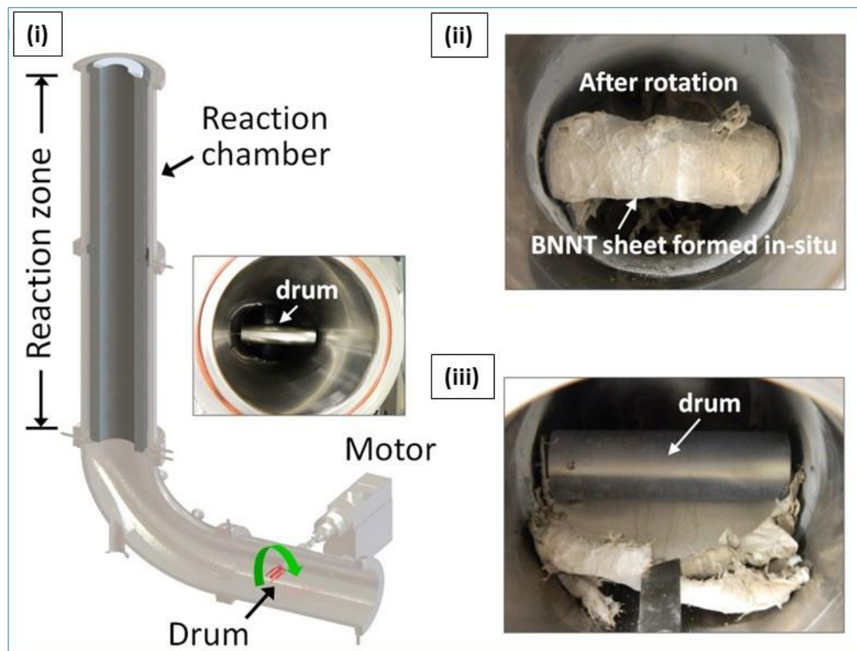
Figure 21. A prototype in-line, dry separation system developed by NRC-C [ref. 28]: (i) a small, rotating drum mounted in the exhaust near the reactor exit; (ii) synthesis product collected on the drum; and (iii) peeling of BNNT sheet material from the drum.
