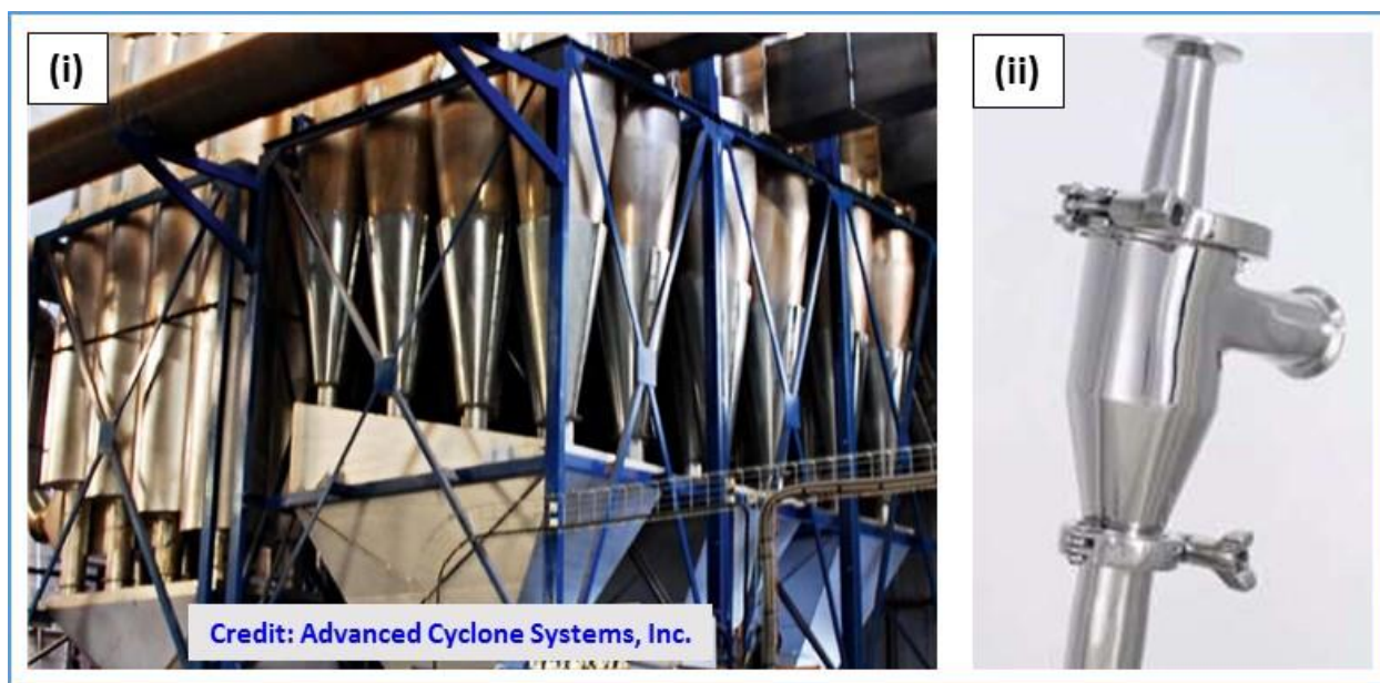
Figure 23. Application spectrum of cyclone technology for nano-particulate collection by ACS, Inc.: (i) emission control—large, multiple units designed for high volume and/or high temperatures [ref. 46]; and (ii) product recovery—smaller, individual units designed for efficiency and cleanliness [ref. 47].
