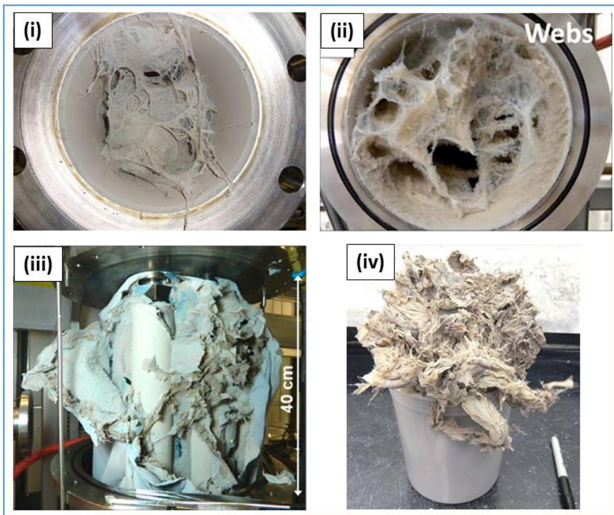
Figure 4. Accumulation of bulk product during the incumbent RF plasma synthesis processes: (i) in the UC-B reactor [ref. 12]; (ii) in the NRC-C reactor [ref. 15]; (iii) in the NRC-C filtration system [ref. 18]; and (iv) BNNT materials weighing ~20 g, manually extracted from the NRC-C filters [ref. 15].
